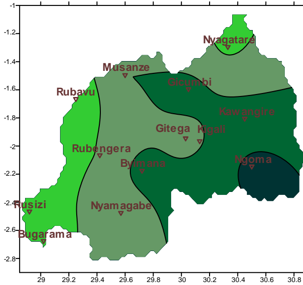
Ikarita ya1: Imvura yaguye (mm): Gicurasi_2017
