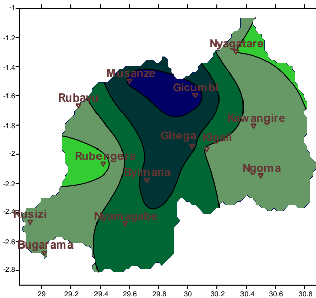
Ikarita ya3: Imvura yaguye (mm): Mata_2017
